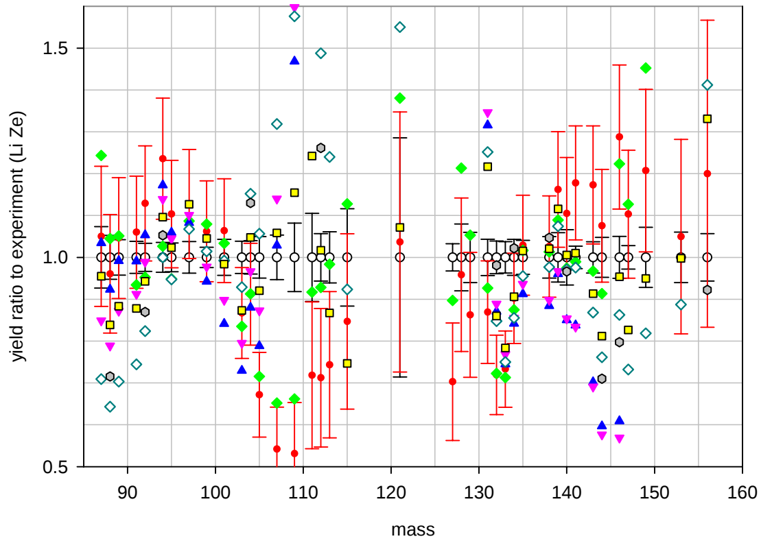
Benchmark A: ^{238}\text{U} at 10.0-11.3 MeV, post neutron emission yield ratios to experiment (Li Ze) lower graph: partial plot (high values omitted, for legend see upper graph).
